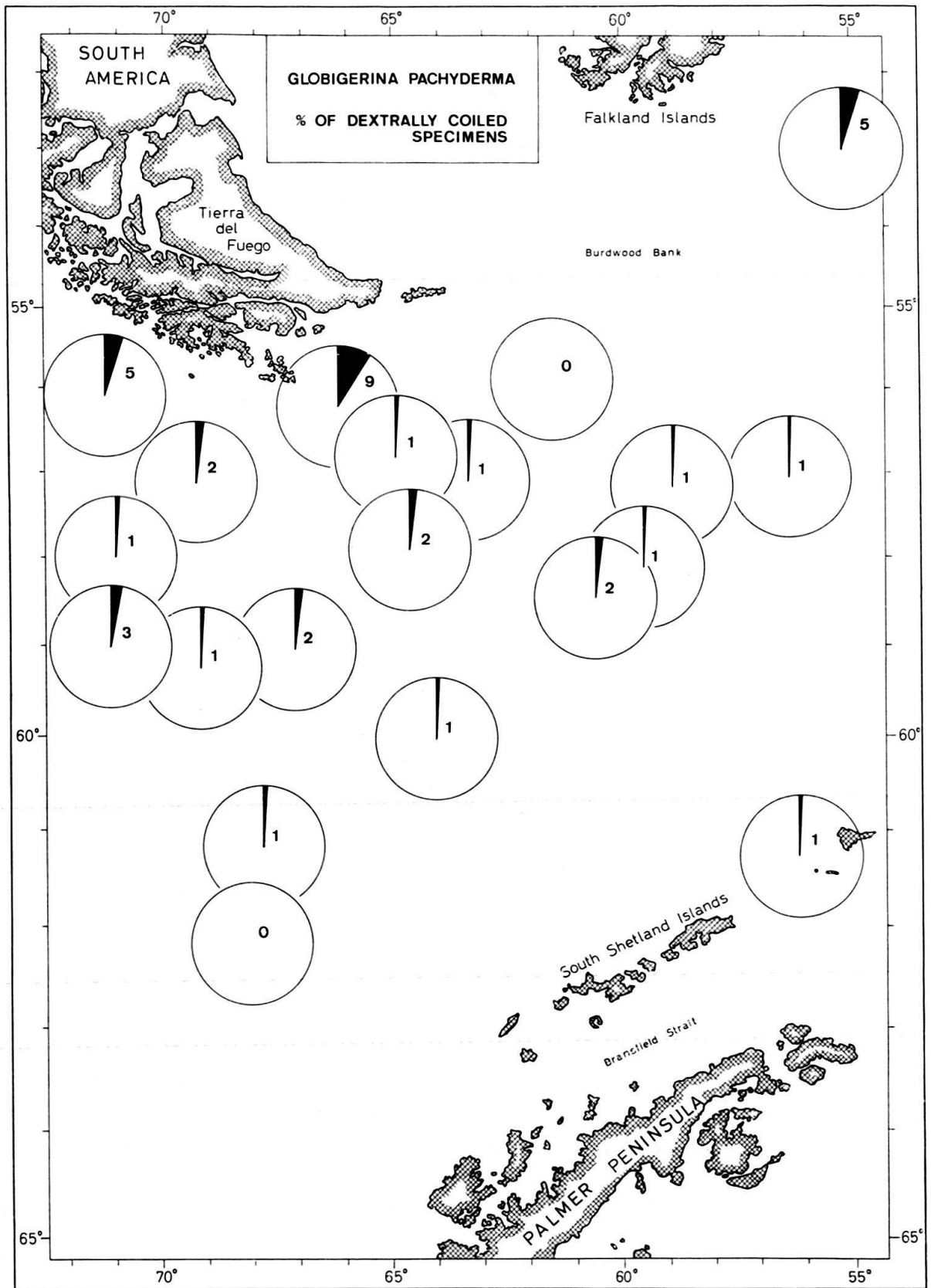
Fig. 2 Distribution of dextrally coiled Globigerina pachyderma (Ehrenberg) in percentages of the total population of this species at each station.
