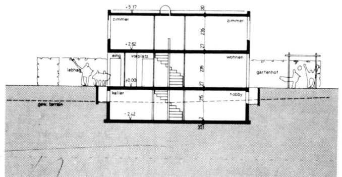
Bruggenmatt development: house cross-sections.
