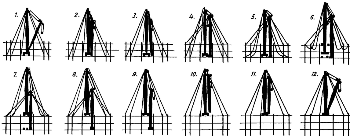
Jumping guy derrick schematic arrangement of sequence
