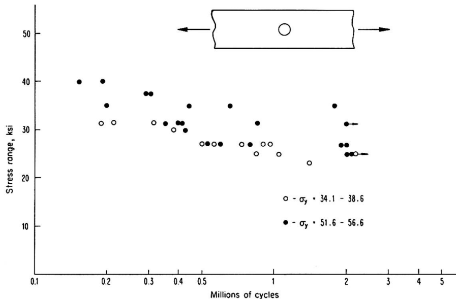
Fig. 1. Fatigue Tests of Plates with Hole.
