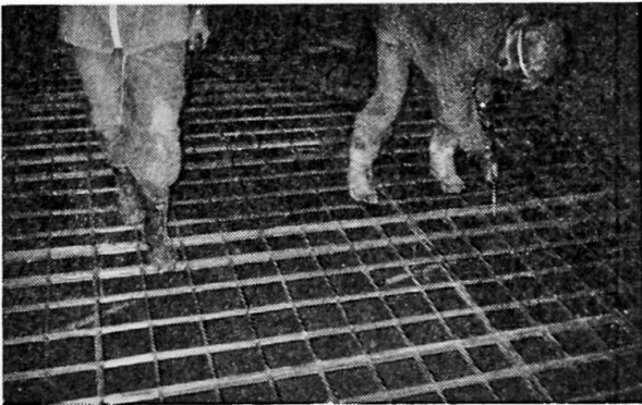
Fig. 5 Reinforcements for invert of concrete lining
