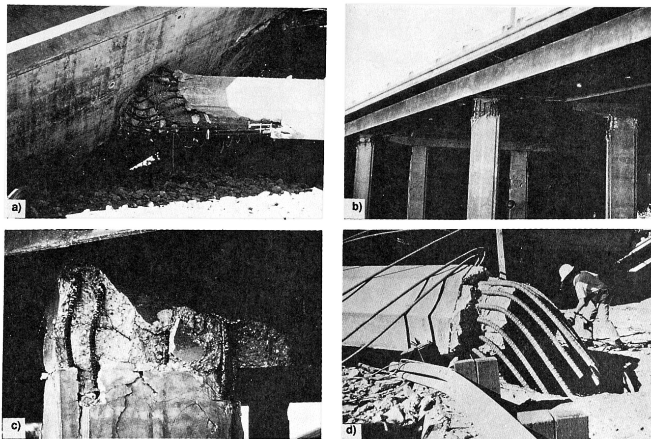
Fig 2. San Fernando Earthquake Bridge Damage (continued)
