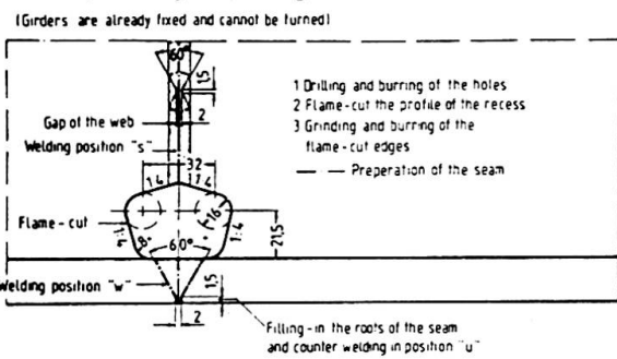
Siteshop welding lower flange with hole
