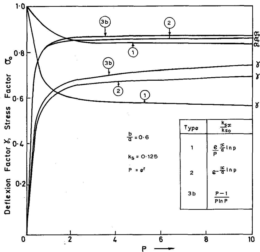
Fig. 2. The effect of foundation modulus reduction parameter p on deflexions and stresses.
