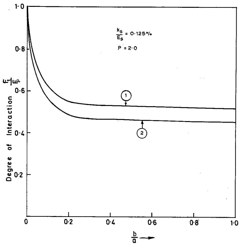
Fig. 4. Degree of interaction against aspect ratio.
