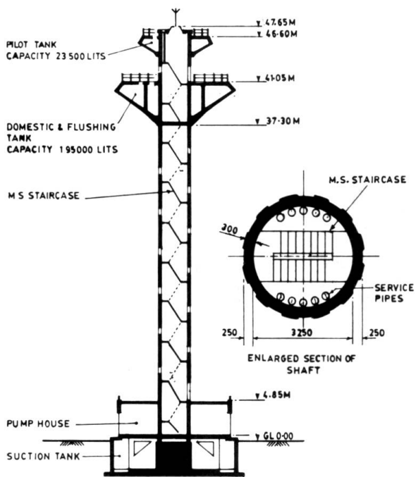
Fig. 1 General arrangement
