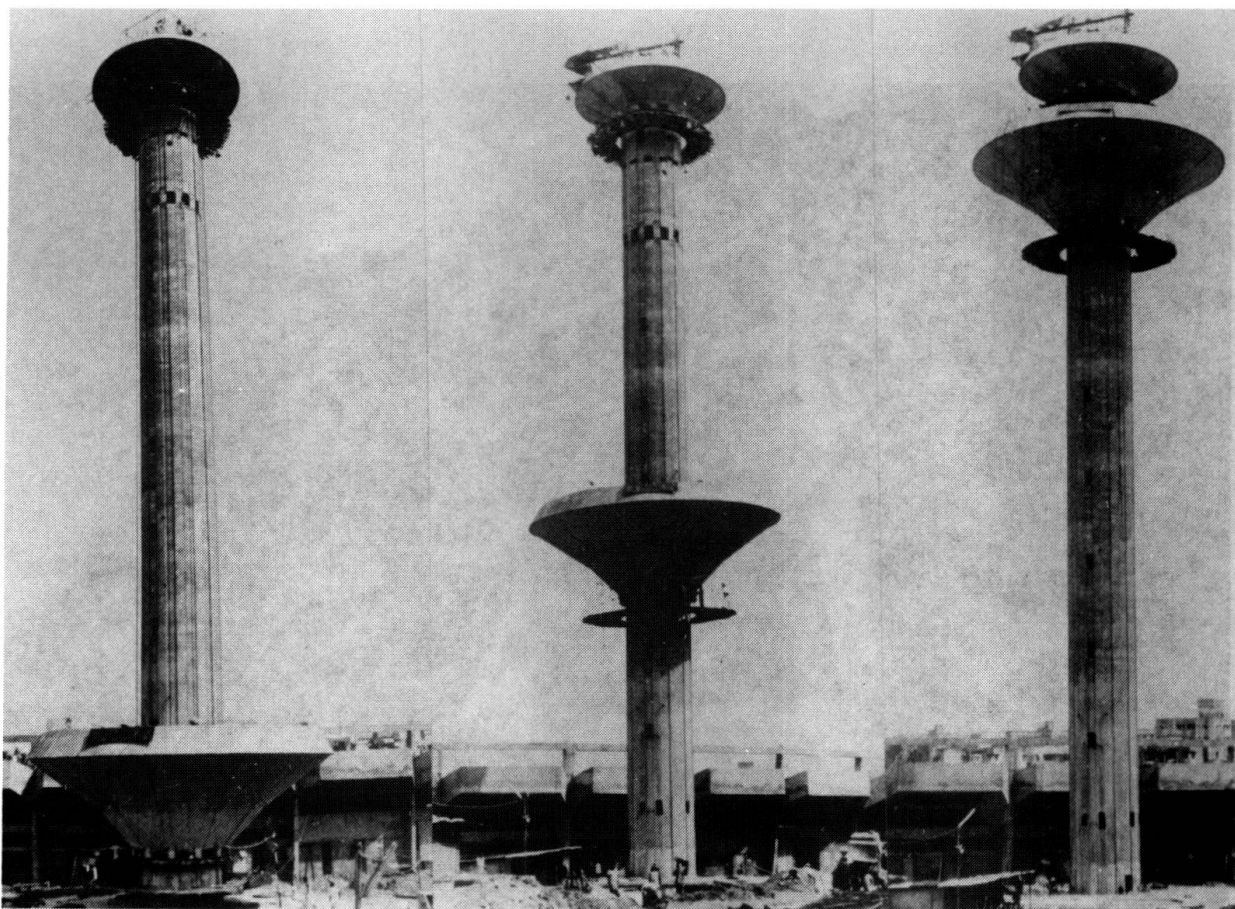
Fig. 2 View during different stages of lifting of the lower tank
