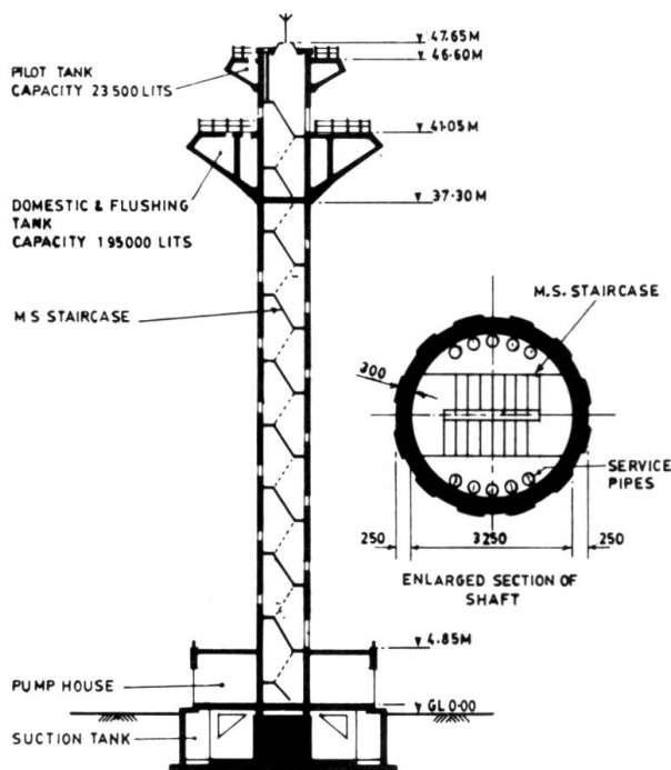
Fig. 1 General arrangement
