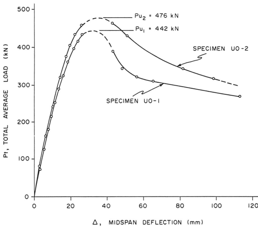
Fig.5 Load-deflection curves
