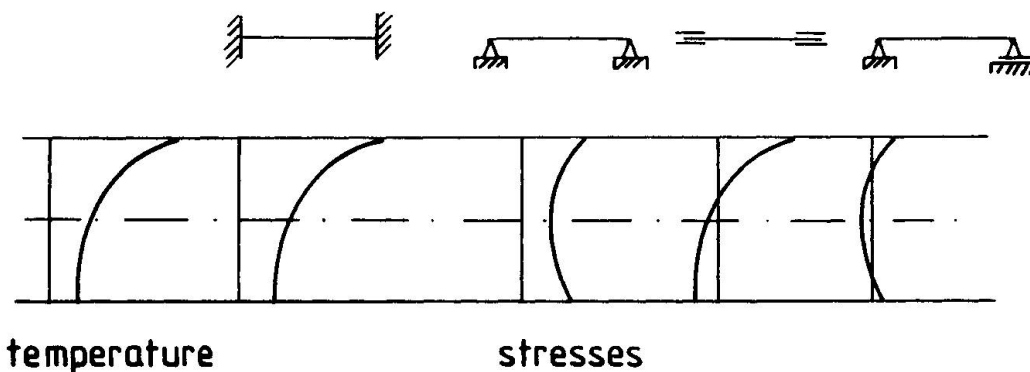
Fig. 1 Stresses due to non-linear temperature distribution with various boundary conditions.
