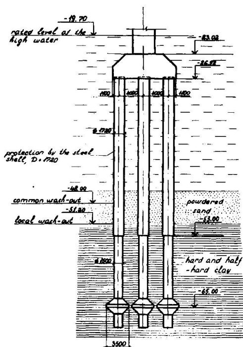
Fig. 1 Pier diagram.
