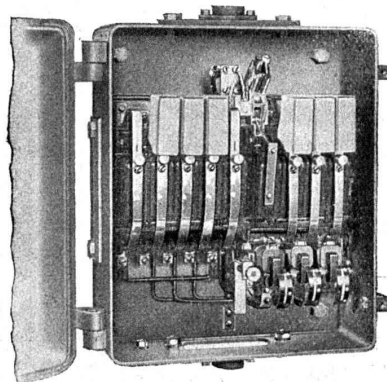
Coffret Type CAY. 15 amp.
