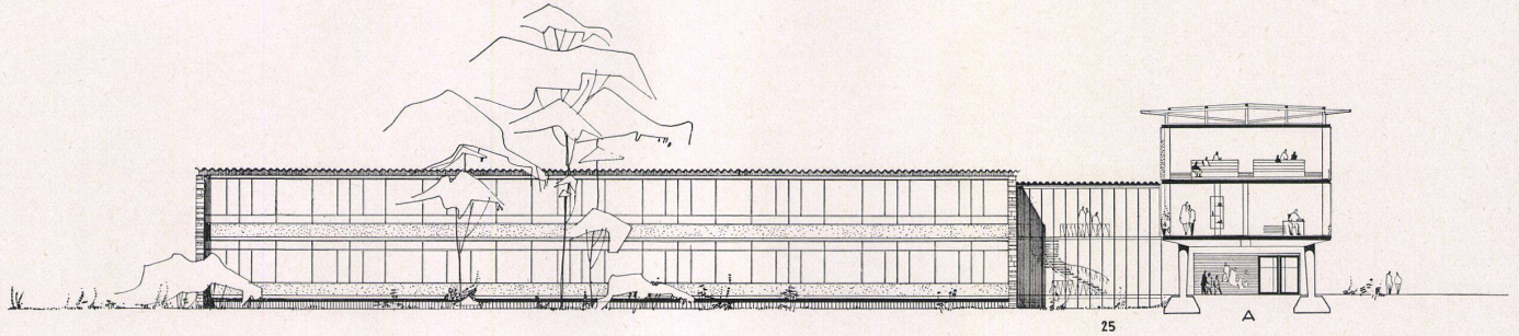
Ostpavillon, Innenhofansicht des Klassentraktes / Pavillon est, aile des classes vue de la cour intérieure / East pavilion, view of class-room structure from interior court 1:450
