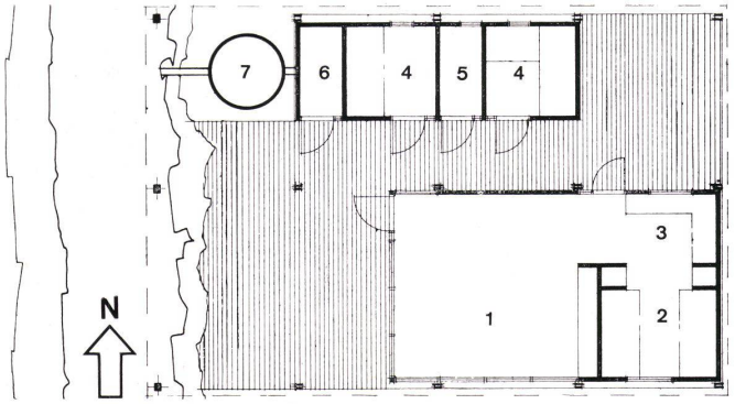
Grundriß Erdgeschoß 1:150.
