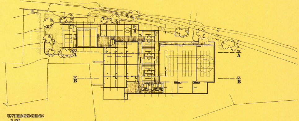
ERDGESCHOß • 0.00 - 402.30 MÜLL.
