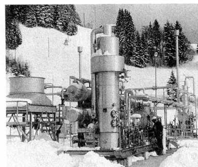
◁ Our own natural gas from the Entlebuch: Drilling site Finsterwald.
