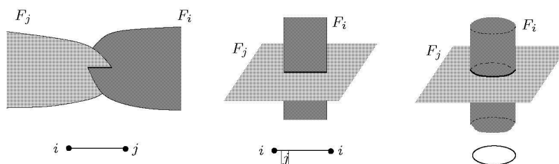
Fig. 5. The three types of intersections F_i \cap F_j : a clasp, a ribbon and a circle.
