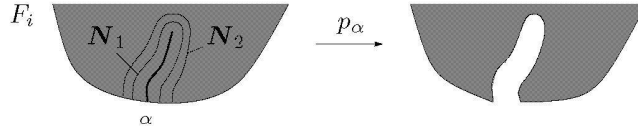
Fig. 2. Push in F_i along an arc \alpha .
