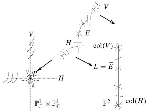
Figure 9. Passing from \mathbb{P}^1_{\mathbb{C}} \times \mathbb{P}^1_{\mathbb{C}} to \mathbb{P}^2 .
