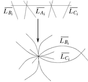
Figure 8. Contraction producing the point r_{A_i} of \mathbb{P}^1_{\mathbb{C}} \times \mathbb{P}^1_{\mathbb{C}} .
