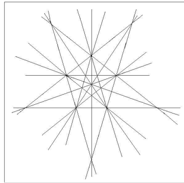
Figure 6. The icosahedral configuration of lines.
