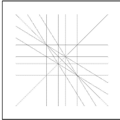
Figure 1. Real picture of the arrangement of lines invariant by \mathcal{H}_5 and \mathcal{H}_9 . The line at infinity is also invariant.
