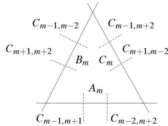
Figure 4. Intersections between diagonals C_{ij} and cycles, with integers taken modulo 5.
