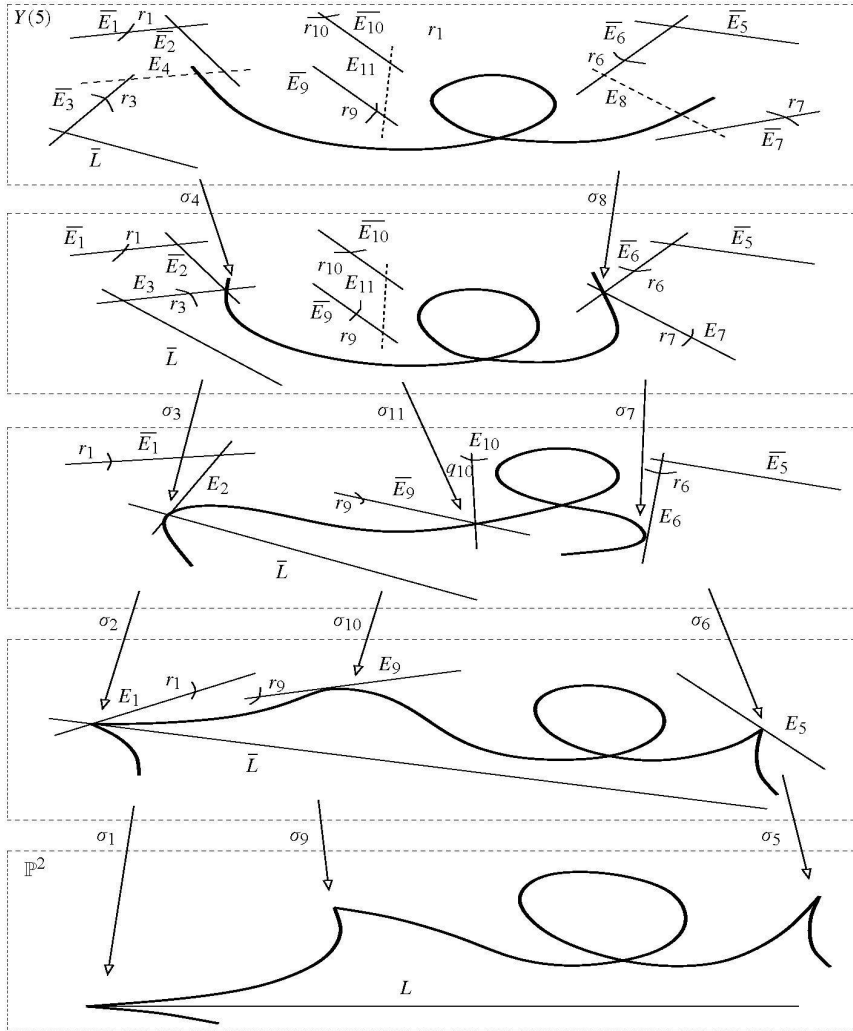
Figure 18. Resolution of \mathcal{H}_3 .
