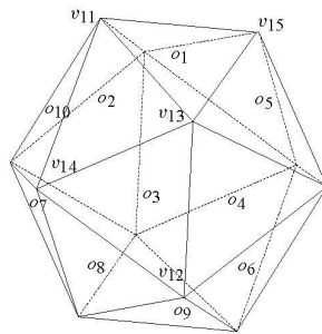
Figure 5. Vertices and centers of faces of an icosahedron.
