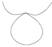
Figure 14. Double cusps of Klein degree 10 curve at the points v_i, i = 11, \dots, 16 .
