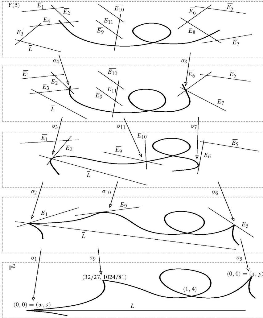
Figure 10. The 11 blow ups composing f: Y(5) \rightarrow \mathbb{P}^2 .
