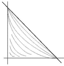
Figure 2. The qualitative behavior of \mathcal{H}_5 and \mathcal{H}_9 on each cell.
