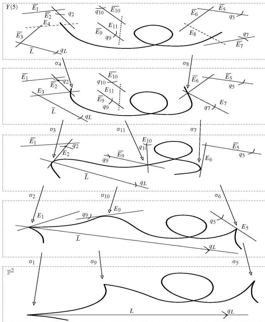
Figure 17. Resolution of \mathcal{H}_2 .
