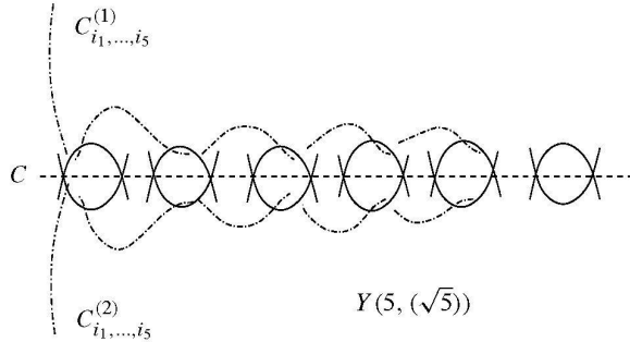
Figure 16. Curves C_{i_1, \dots, i_5}^{(1)} and C_{i_1, \dots, i_5}^{(2)} are pre-images of \bar{C}_{i_1, \dots, i_5} .
