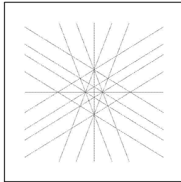
Figure 7. The arrangement of lines induced by the icosahedron, with one line at infinity.
