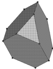
Figure 3. Polytope P .
