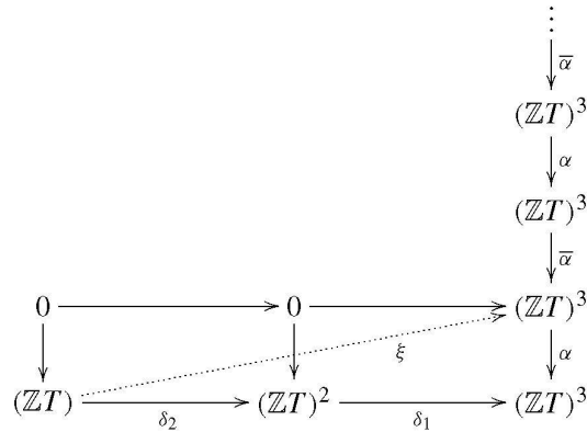
Figure 2. System of free \mathbb{Z}T -modules.
