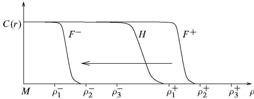
Figure 1. The functions F^\pm and the homotopy.
