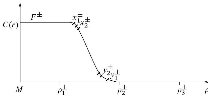
Figure 2. The energy levels x_l^\pm and y_l^\pm .
