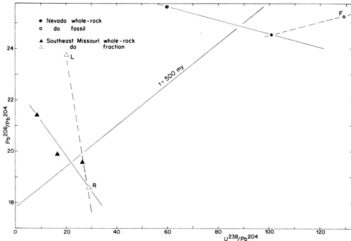
Fig.1. ^{206}\text{Pb}/^{204}\text{Pb} - ^{238}\text{U}/^{204}\text{Pb} isochron diagram for samples from Nevada and Missouri. Solid line is 500 m.y. isochron using a 500 m.y. old model lead as the initial lead. Dashed lines connect analyzed fractions of a rock with their whole rock: L- is the 6N-HCl soluble fraction and R is the residue from the acid leach; F is the inarticulate brachiopod fossils.
