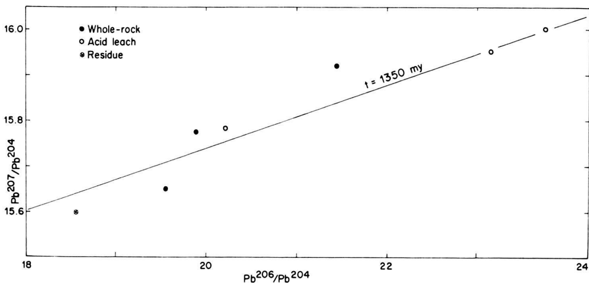
Fig.2. ^{207}\text{Pb}/^{204}\text{Pb} versus ^{206}\text{Pb}/^{204}\text{Pb} isochron diagram for samples from Southeast Missouri. Isochron is drawn for the age of the basement in the area. Acid leach is with 6N-HCl and residue is that fraction not dissolved by the acid.
