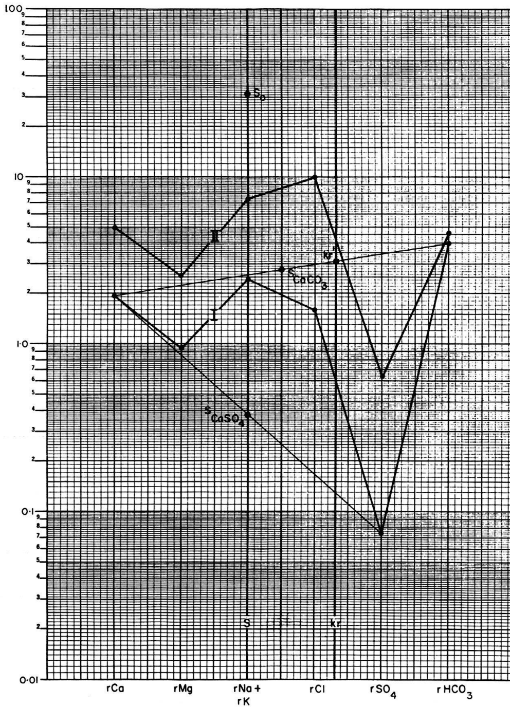
Fig. 4. Chemical analyses: Average values in epm for group I (10 wells) and group II (9 wells) with calculated S_0 , S_{CaSO_4} , S_{CaCO_3} , kr' for group I.
