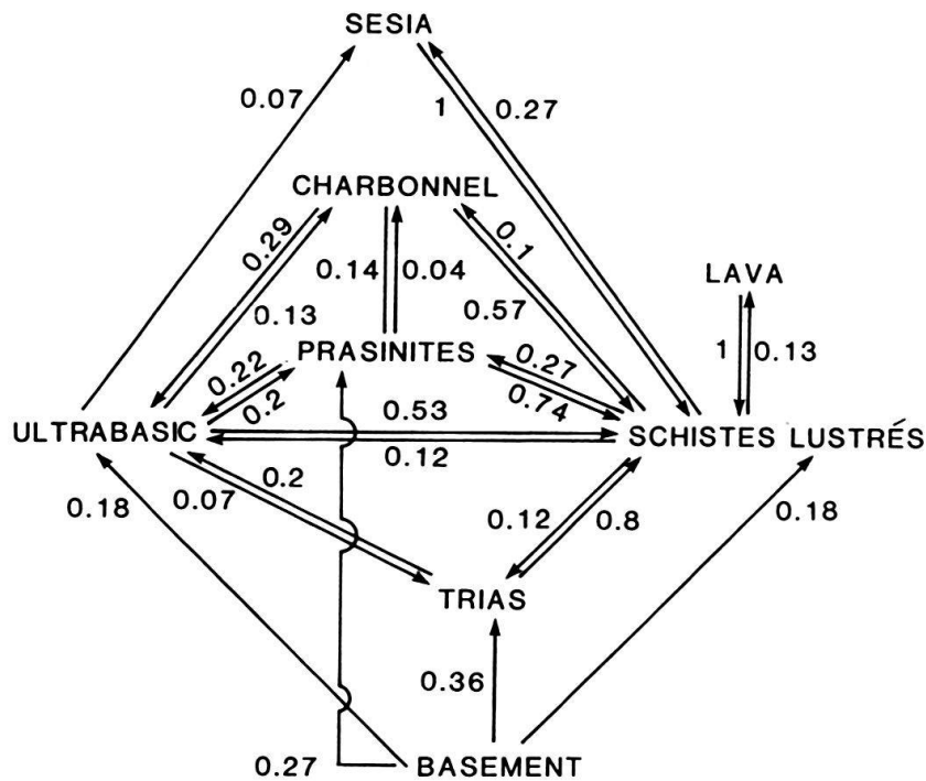
Fig. 12. Transition frequency matrix, transition probability matrix and transition probability diagram for all transitions, the Gran Paradiso region. For discussion see text.
