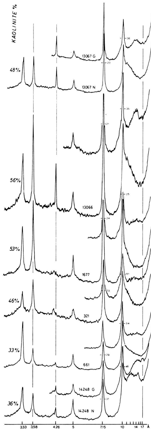
Fig. 13. Diffractograms of oriented samples, air dried (N), and treated with ethylene glycol (G). Source: Cu K\alpha , Philips apparatus, specifications: see PERSOZ (1982). Samples are from Hauptmumienbank and Geissberg Members: 14248 Courgenay, 661 Foradrai, 321 Pichoux, 1677 Reuchenette, 13066-67 Aargau.
