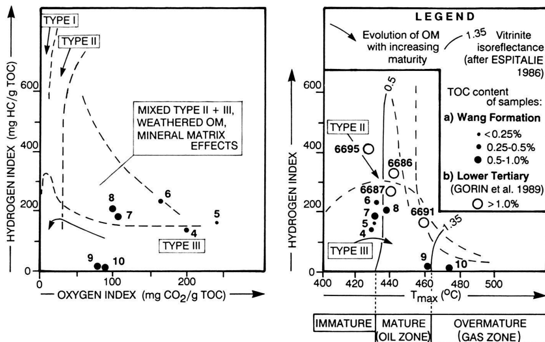
Fig. 3. Rock-Eval pyrolysis results: classification of organic matter in a HI-OI diagram and display of thermal maturity variations in a HI- T_{\max} diagram. Mineral matrix effects may affect HI, OI and T_{\max} values of samples 4 to 10. In particular, OI for samples 4, 5 and 6 may be too high because of their low TOC content (<0.5%).
