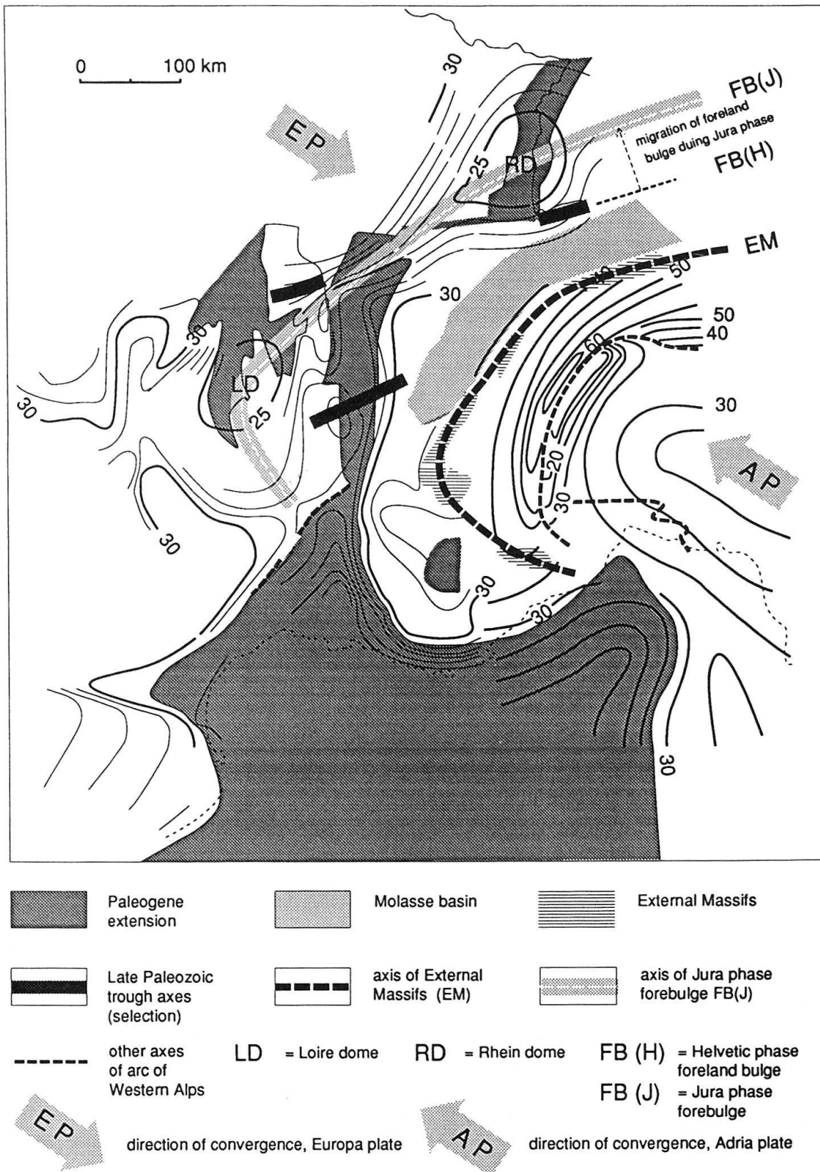
Fig. 14. The estimated positions of the foreland bulges attributable to the Helvetic-Insular phase (FBH) and the Jura phase (FBJ), superimposed on the isobaths of the Moho (after Hirn 1980, Giese). Very dark bands: examples of known late Paleozoic troughs. Dark shading: Paleogene to Early Miocene extensional structures.
