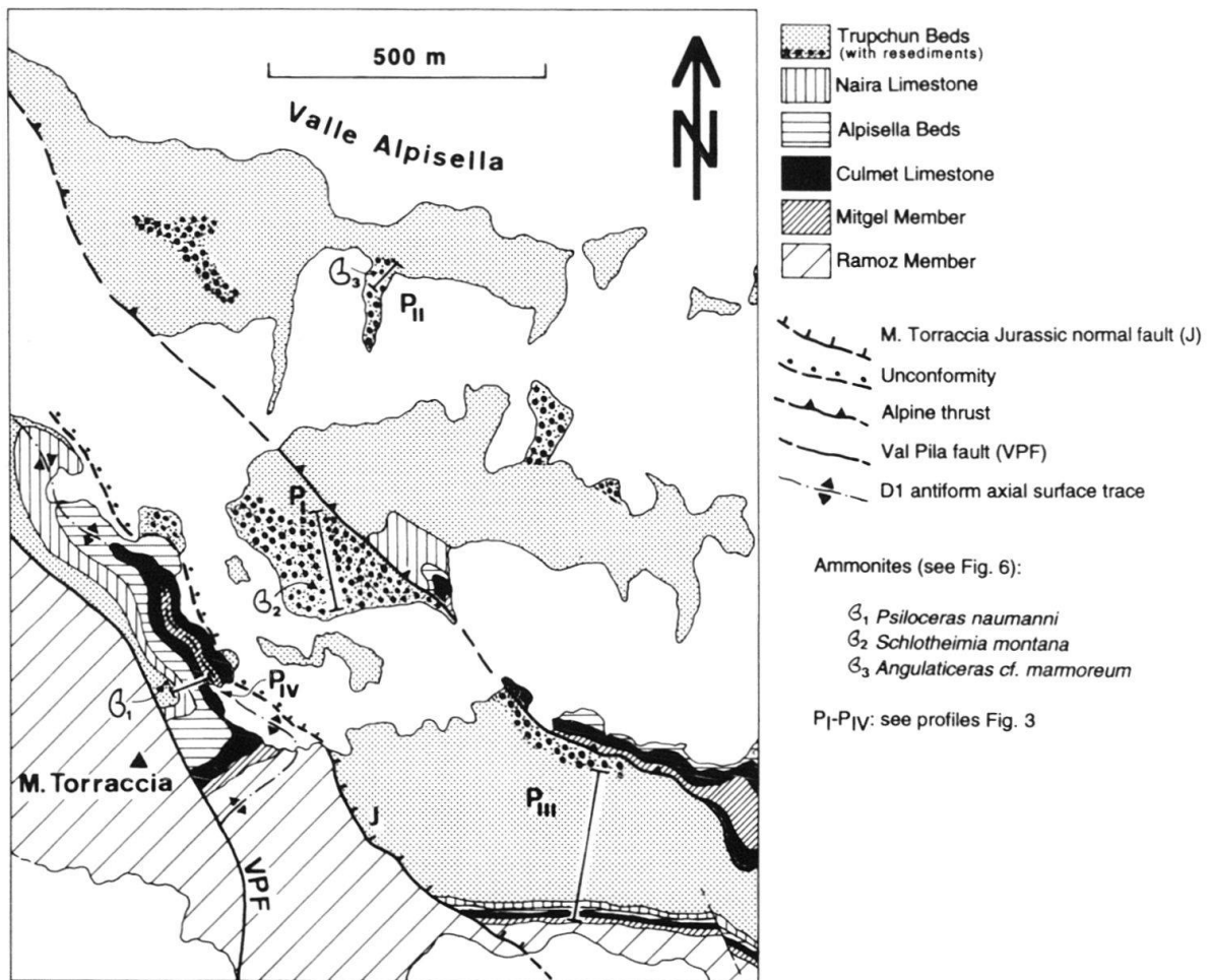
Fig. 7. Geological map of the M. Torraccia area.
