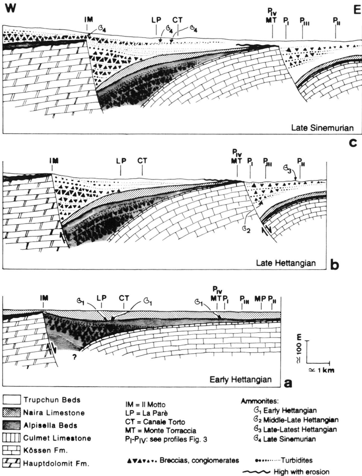
Fig. 9. Evolution of the Il Motto and M. Torraccia basins based on ammonite finding and sedimentological observations.
