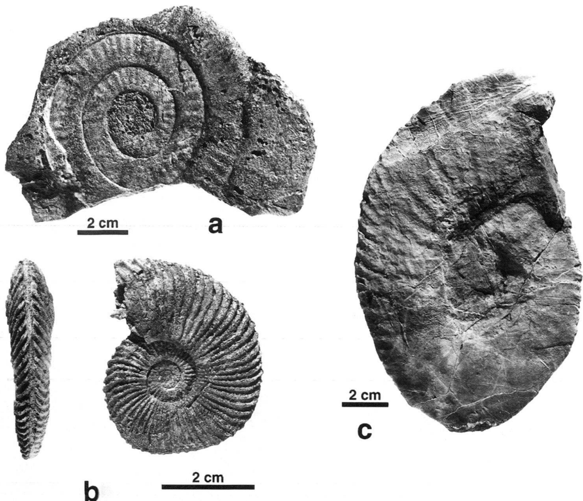
Fig. 5. Ammonites from the M. Torraccia-Valle Alpisella area; see Fig. 3 and Fig. 7 for locations. a) Psiloceras naumanni (NEUMAYR), Alpisella Member, north of M. Torraccia, Swiss coord. 812.700/158.150, 2640 m a.s.l.; b) Schlotheimia montana (WAEHNER), Trupchun Beds, north of M. Torraccia along profile P I , Swiss coord. 812.900/158.250, 2550 m a.s.l.; c) Angulaticeras cf. marmoreum (OPPEL), Trupchun Beds, Valle Alpisella along profile P II , Swiss coord. 812.750/158.875, 2335 m a.s.l.
