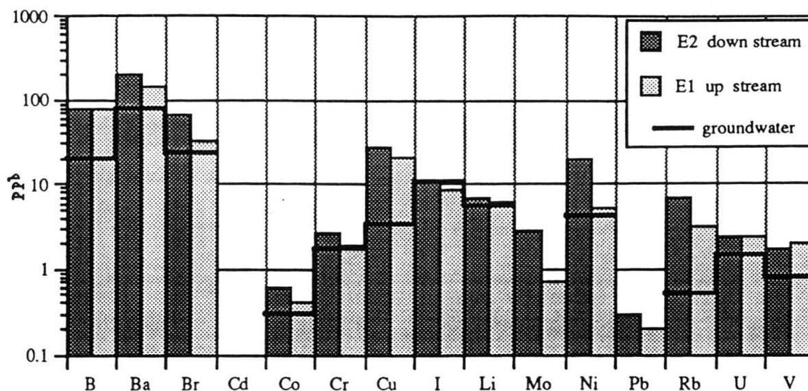
Fig. 6 Multi-elemental analysis for down-stream and up-stream near an old waste site compared to groundwater sample.
