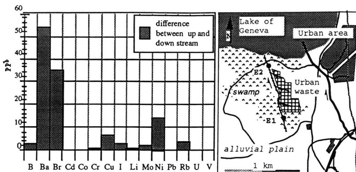
Fig. 7. Concentrations difference between the up- and down-stream samples and their situations.
