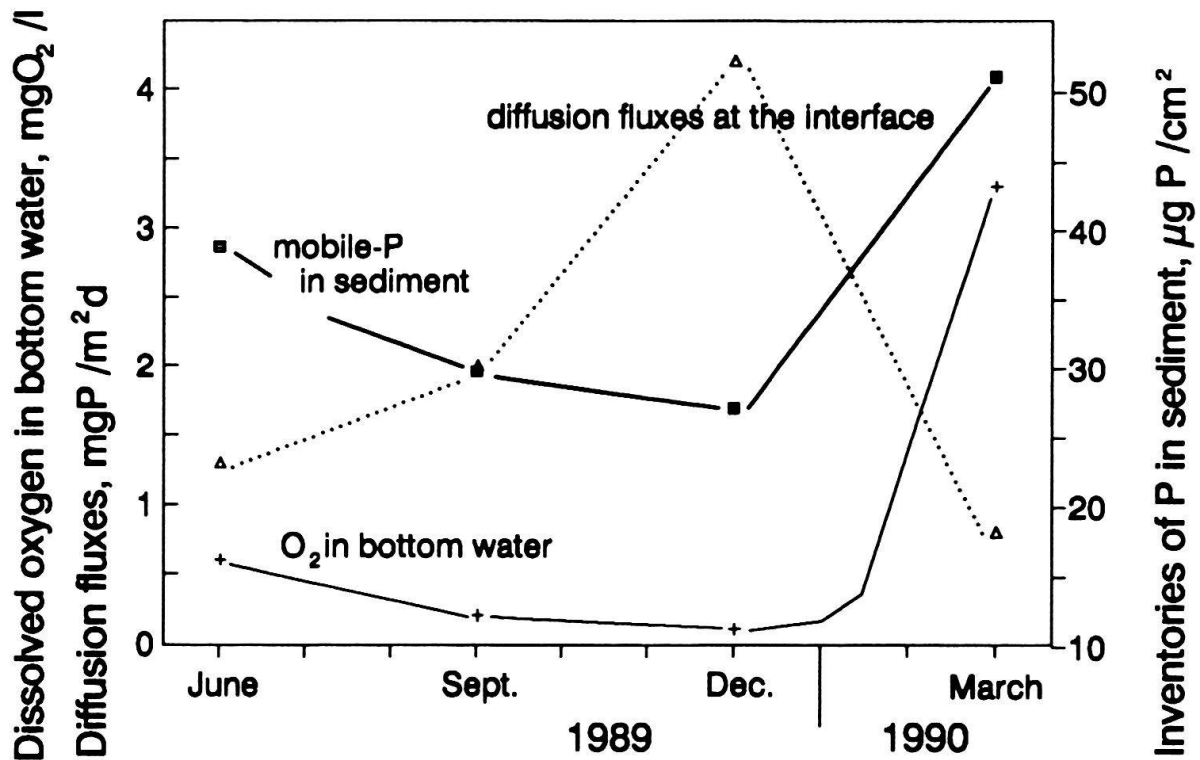
Fig. 6. Relationship between mobile-P (NAI-P and O-P) in surficial sediments, diffusion fluxes of soluble P at the interface and dissolved oxygen concentrations in bottom water in site Melide (data from LSA for dissolved oxygen content).
