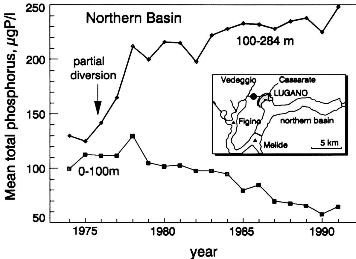
Fig. 3. Influence of a partial diversion of municipal sewage on total phosphorus in the northern basin of Lake Lugano. Data are given for the epilimnion and hypolimnion (data from LSA 1992).
