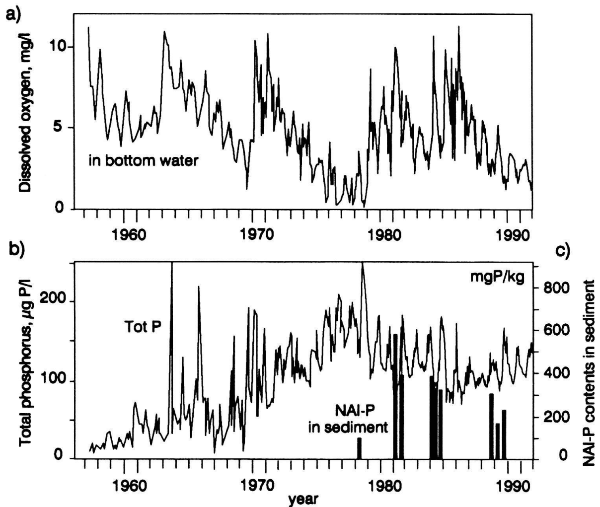
Fig. 5. Dissolved oxygen (a) and total phosphorus (b) in bottom water of Lake Geneva (data from CIPEL) and NAI-P content (c) in surficial sediments (same sampling station 307 m depth).
