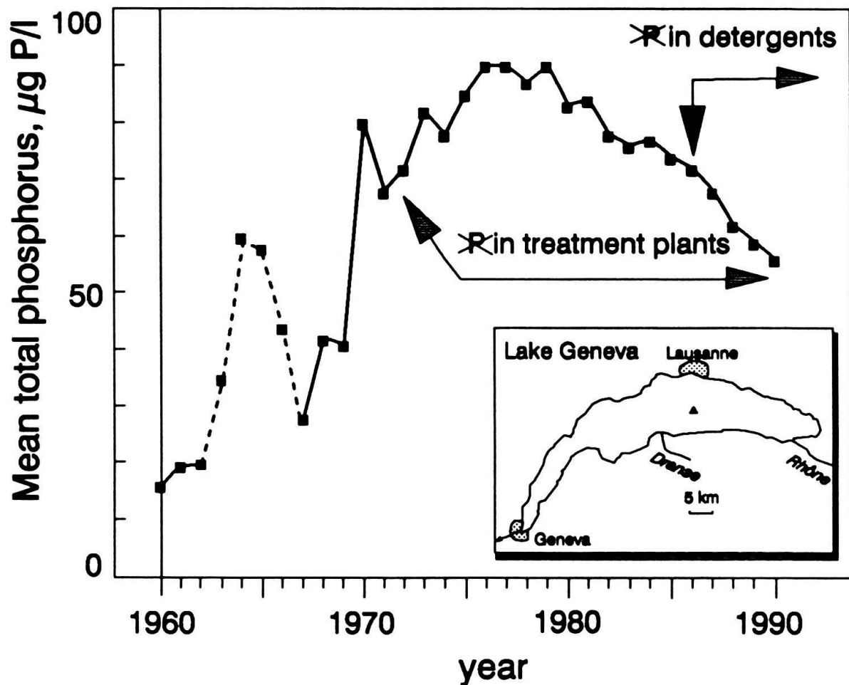
Fig. 4. Influence of two basic strategies used for reducing nutrients in Lake Geneva on the total phosphorus in the water column (data from CIPEL).
