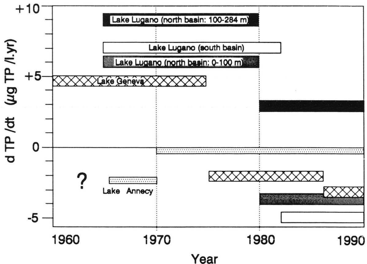
Fig. 7. Total phosphorus rates of accumulation in different sub-basins of the studied lakes from 1960 to 1990 (see text for explanation).
