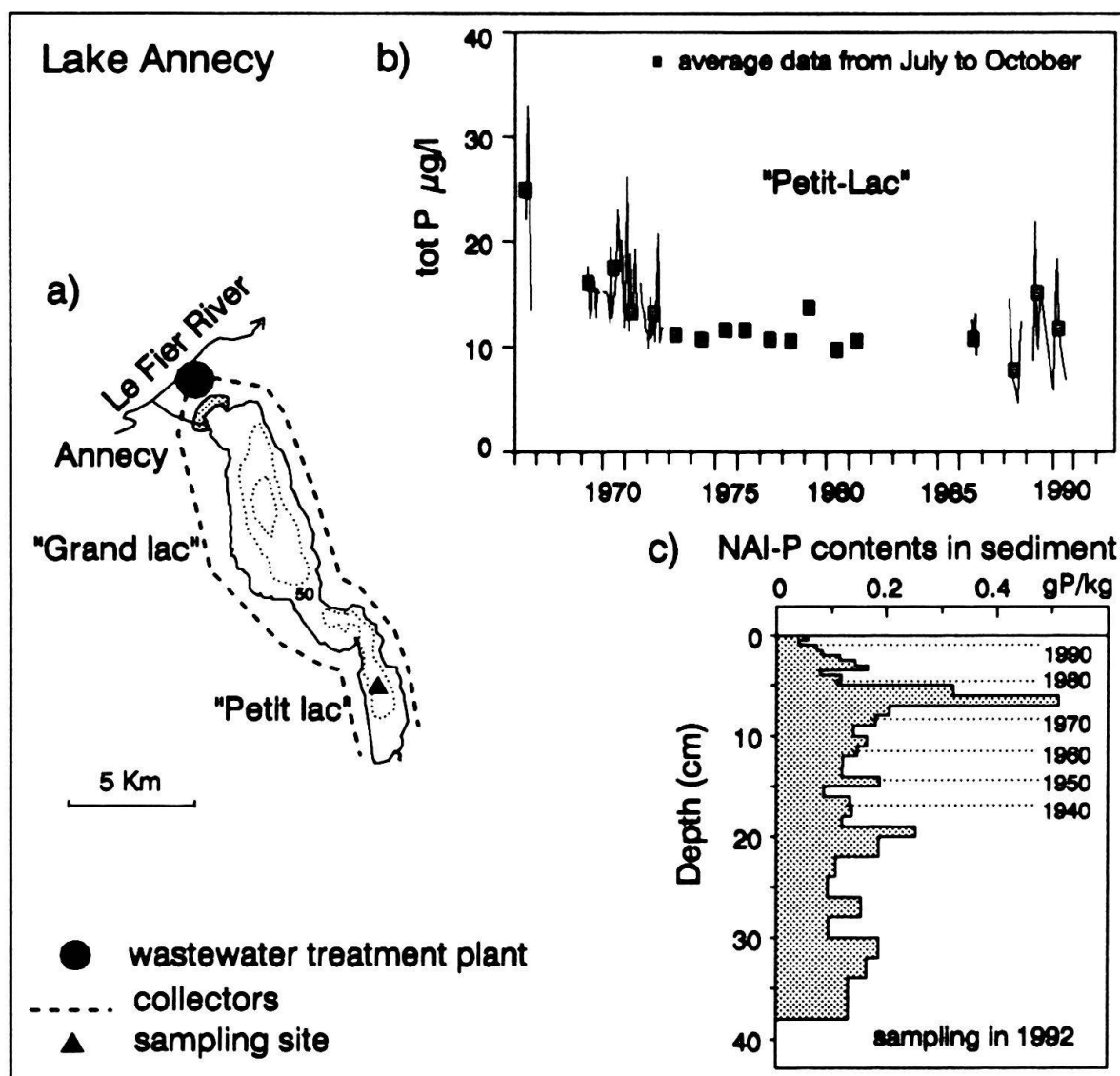
Fig. 2. Schematic diagram of the complete diversion of effluent in Lake Annecy performed in early 1970's (a), P-response in the water column (data from SILA) (b) and in sediments (c). Dating is based on ^{137}\text{Cs} profile in sediment (unpublished results from Institute F.-A. Forel).
