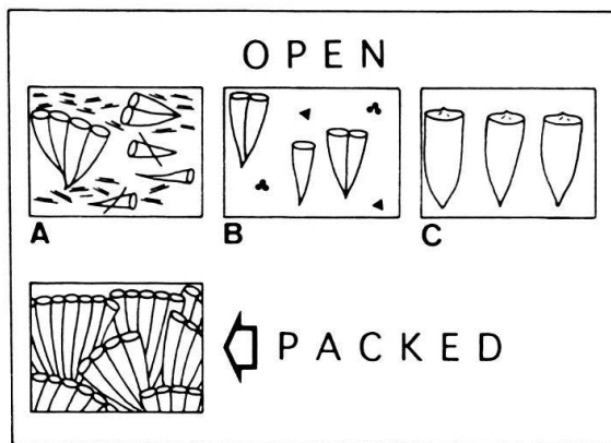
Fig. 7. Types of biostrome fabric. The open fabric is matrix-supported, and the rudists or rudist clusters are not in contact with each other. Three varieties of open fabric are distinguished. A: open fabric with a matrix of bioclastic grainstone to rudstone. B: open fabric with a matrix of wackestone to floatstone (with miliolids, blackened bioclasts, microbial lumps and ostracods). C: open fabric with a matrix of well-sorted, fine bioclastic grainstone to packstone between large radiolitids ( Durania , Joufia ). In the packed fabric, the rudist clusters are in contact with and support each other, and little space is left for matrix.
