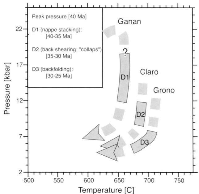
Fig. 15. P-T paths for the three localities discussed in the text and inferred P-T conditions associated with a particular deformation phase at each locality. Pressures reflect progressive exhumation during D1-D3, while increasing temperatures are apparent and reflect different starting temperatures for the three localities.
