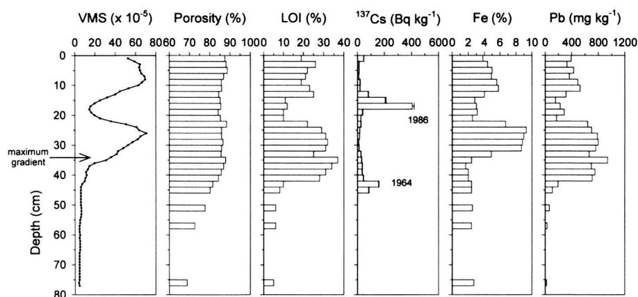
Figure 4. Sediment core E6. Profiles of VMS, porosity, LOI (organic matter), ^{137}\text{Cs} activity, and concentration of Fe and Pb. The two ^{137}\text{Cs} activity peaks correspond to the bomb test (1964) and Chernobyl accident (1986). The increase of VMS is defined as the layer presenting the maximum gradient. Pb concentration profile presents a sharp increase corresponding to the start of the sewage treatment plant of Lausanne (1964), whereas Fe increases simultaneously with VMS, both resulting from the implementation of a chemical stage in the STP using \text{FeCl}_3 .
