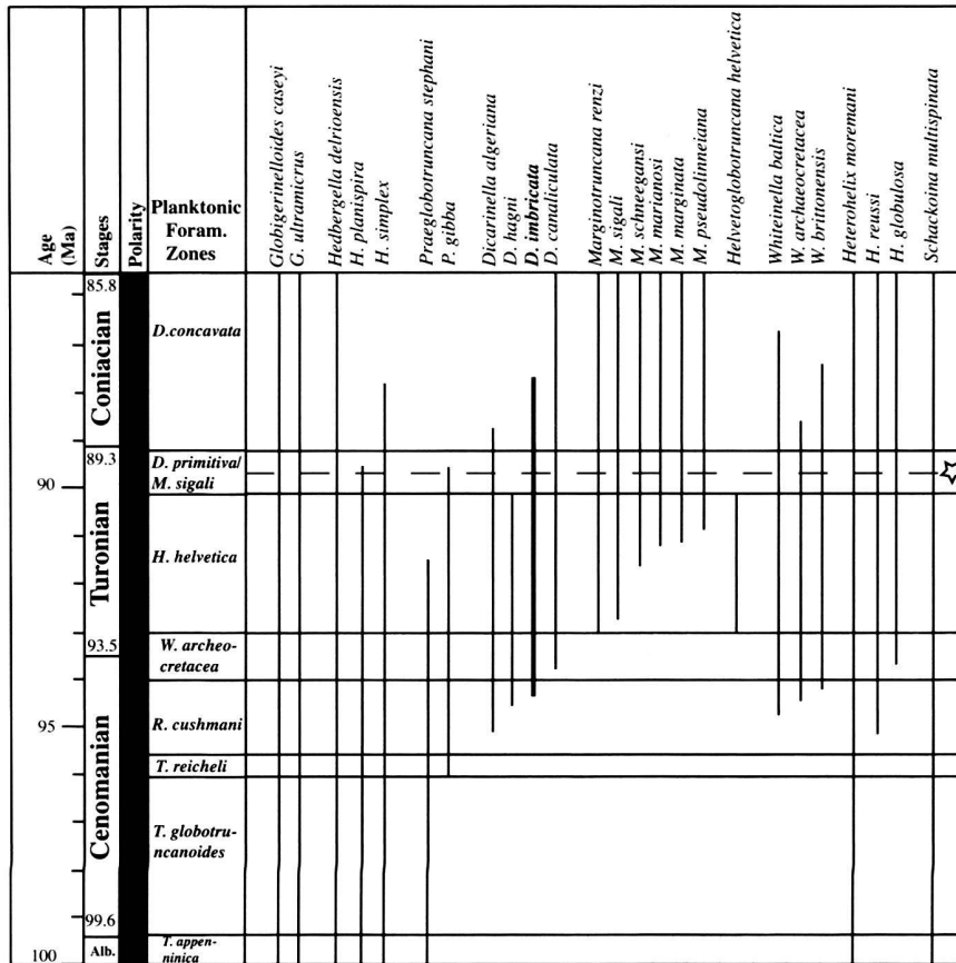
Fig. 1. Stratigraphic distribution of Upper Cretaceous genera and species of planktonic foraminifers from the type horizon of Dicarinella imbricata (MORNOD 1949). The star marks the suggested position of the type level of Dicarinella imbricata , according to the faunal analysis (see text: 5. Accompanying assemblage). Time scale from Ogg et al. (2004).
