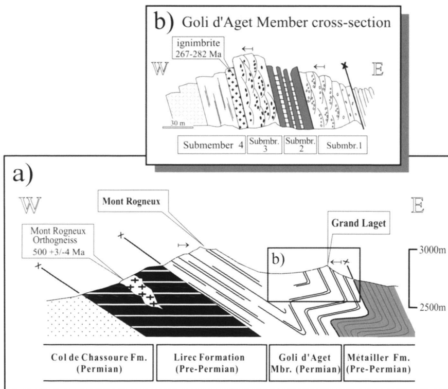
Fig. 2. a) Tectonic units of the "Grand Saint-Bernard nappe" (Briançonnais) in the area of Grand Laget and Mont Rognieux mountains. b) Schematic cross section of the Goli d'Aget Member. Four submembers are distinguished.
