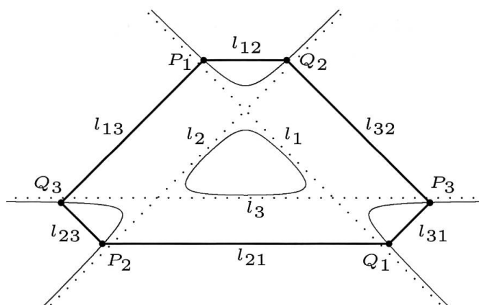
FIGURE 2 Inscribed hexagon H_X
