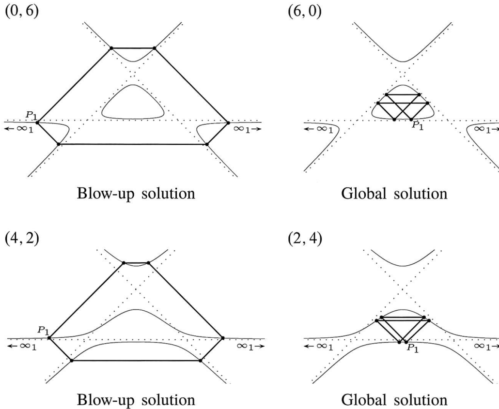
FIGURE 3 Different types of regularly inscribed hexagons and the behavior of the corresponding solutions
