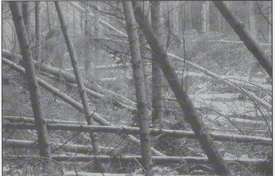
Forest near Berne, damaged by "Lothar" on Dec. 26.99
