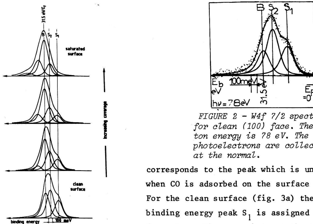
FIGURE 3 - W4f\ 7/2 spectra for increasing coverage of carbon monoxide on (100) face.
