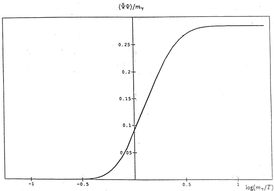
Fig.1: The expectation value of the chiral condensate as a function of the temperature.
