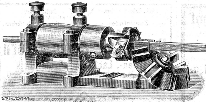
Rundstabhobelmaschine
