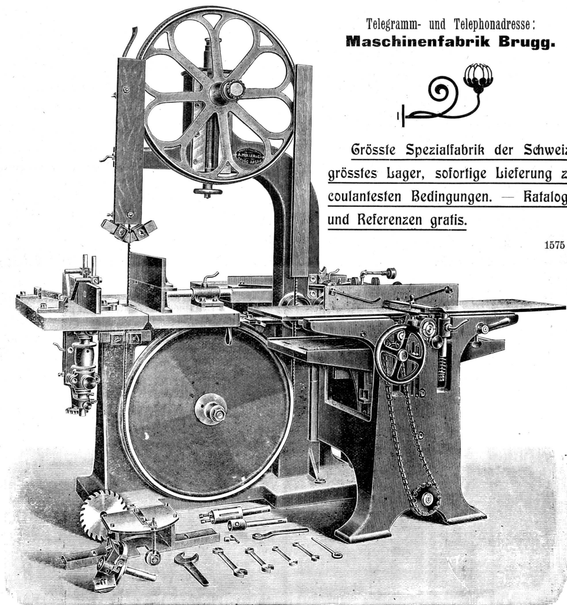
Universalmaschine No. 3.
