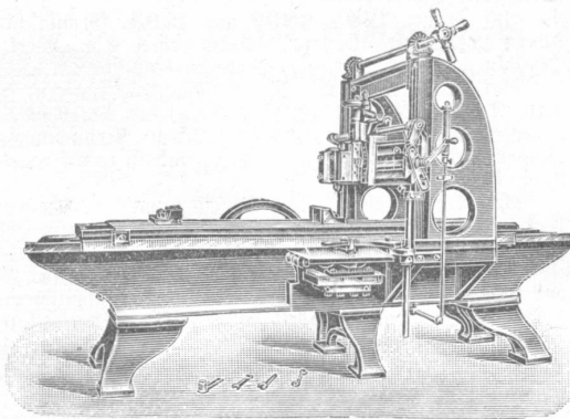
Hobel-Maschine.
