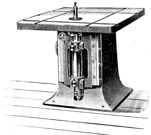
Kehlmaschine.
