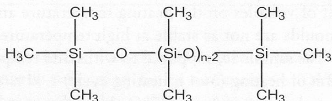
Linear polydimethylsiloxanes (Ln)
