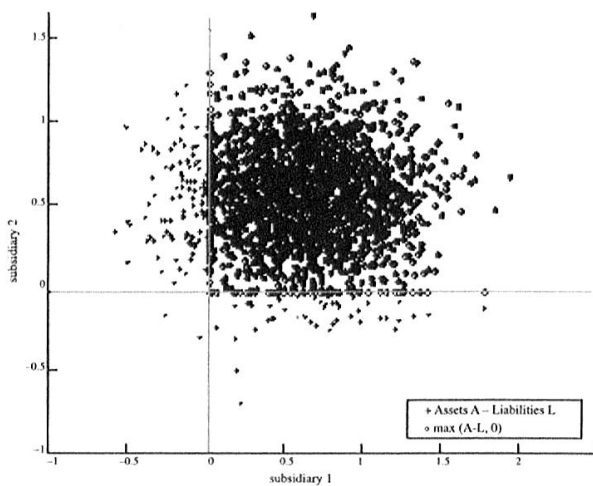
Figure 2 2000 base case sample points of the Monte Carlo simulation. Plus signs are the values of assets - liabilities of subsidiaries 1 and 2. Open circles denote the value of S1 and S2 from the point of view of the holding company. Due to limited liability, these values cannot be negative.
