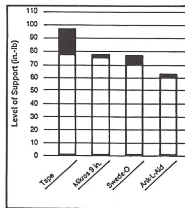
Figure 4: Decrease in ankle support in tape and top three lace-on braces after 20 minutes of inversion cycles
