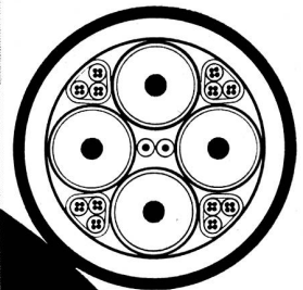
TYPE 2.6/9.5 MM \varnothing
