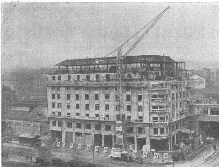
STAHLSKELETT (Hôtel Cornavin, Genf).
