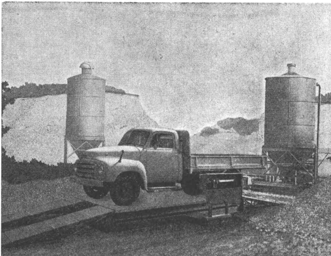
Transportable Baustellenwaage
