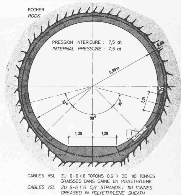
Fig. 4b. Section type tronçons A Typical cross-section A
